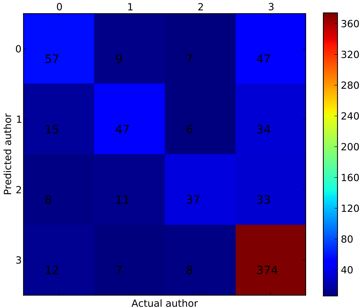
Confusion matrix
